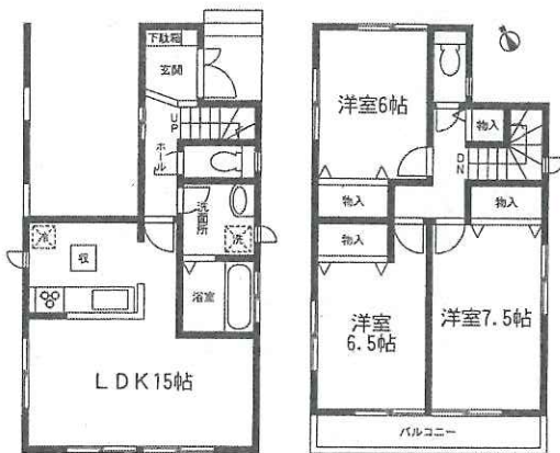
1階平面図:39.75m 2 (12.02坪) 2階平面図:46.38m 2 (14.02坪)
